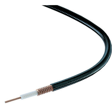
FSJ2-50, HELIAX® Superflexible Foam Coaxial Cable, corrugated copper, 3/8 in, black PE jacket
