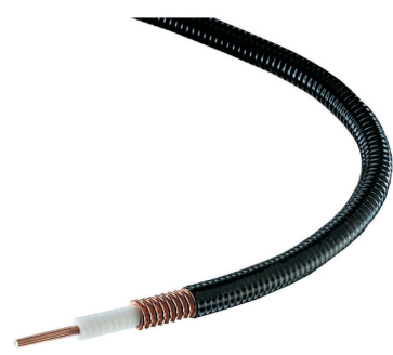
LSF2-50, HELIAX® Superflexible Foam Coaxial Cable, corrugated copper, 3/8 in, black PE jacket (Not for Individual Sale - Jumpers only)
