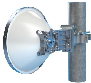
0.3 m | 1 ft ValuLine® High Performance Low Profile Antenna, single-polarized, 12.700–13.250 GHz
