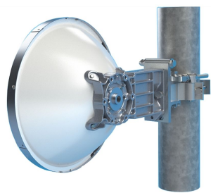
0.3 m | 1 ft ValuLine® High Performance Low Profile Antenna, dual-polarized, 17.700–19.700 GHz
