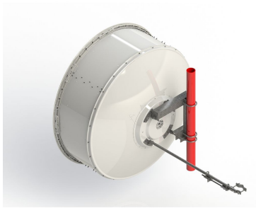
1.8 m | 6 ft ValuLine® High Performance Low Profile Antenna, dual-polarized, 12.700–13.250 GHz
